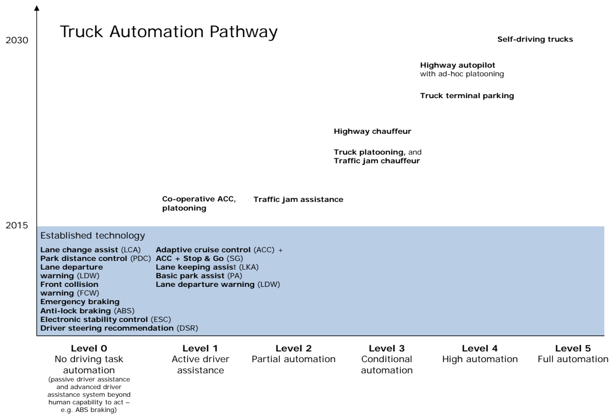
Figure 6. Heavy-duty truck automation pathway from human to fully automated driving
